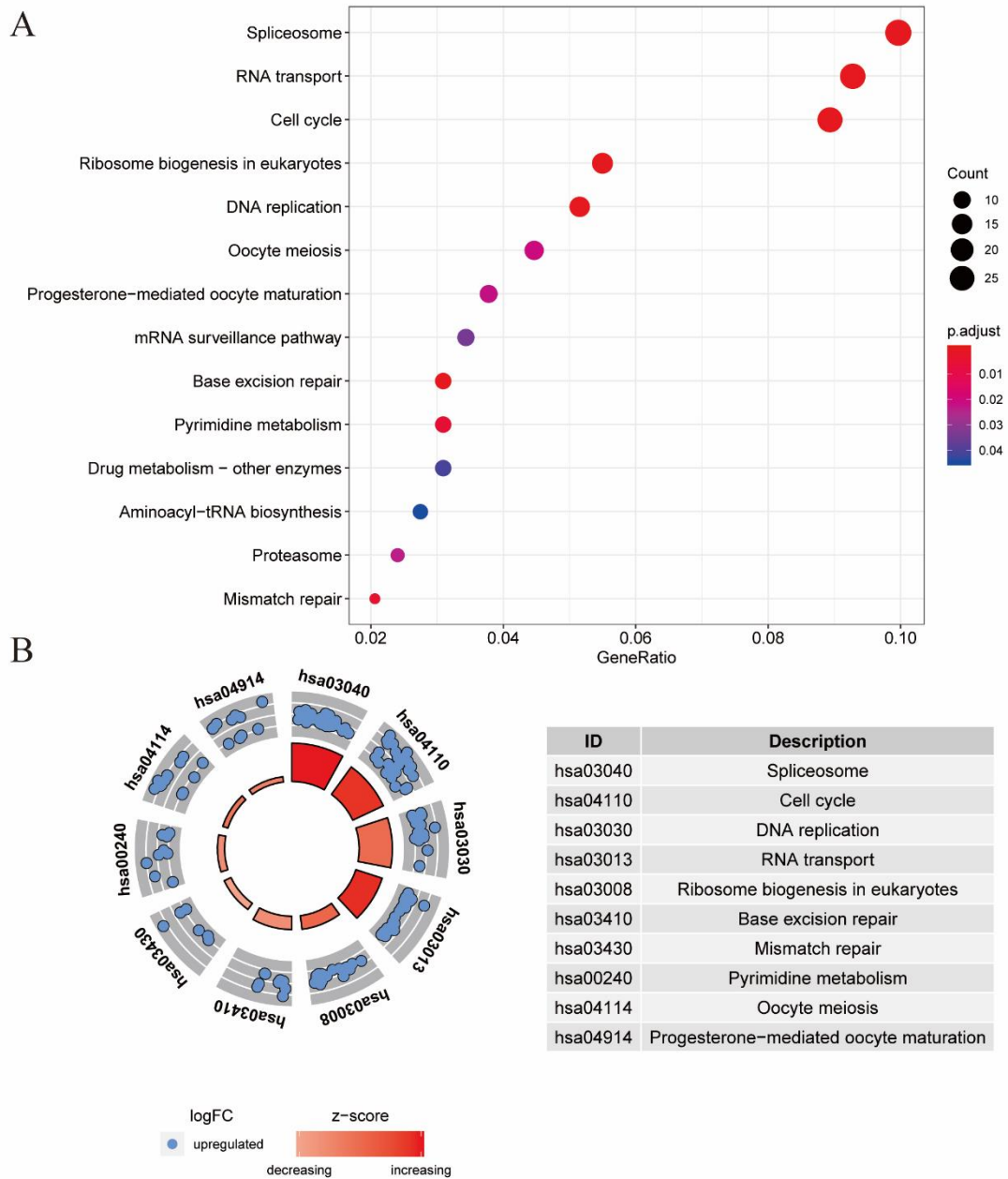
Figure S3. KEGG analysis of co-expressed genes with AATF. KEGG analysis revealed the most important pathways in HCC.
