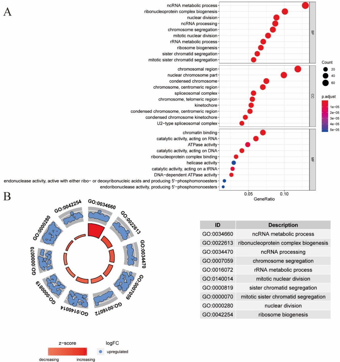
Figure S2. GO enrichment analysis of co-expressed genes with AATF. GO analysis revealed the most significant biological process, molecular function and cell cellular in HCC.
