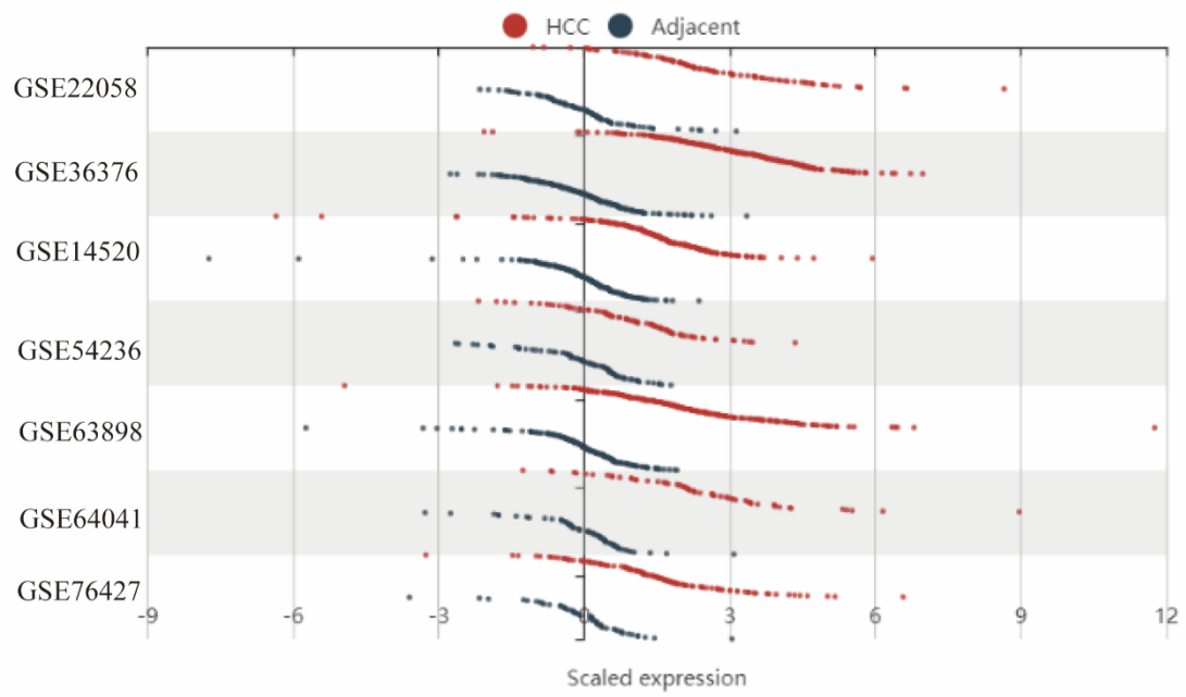
Figure S1. Comparison of AATF expression between HCC and ANTTs in seven GEO series. ANTTs: adjacent non-tumor tissues.
