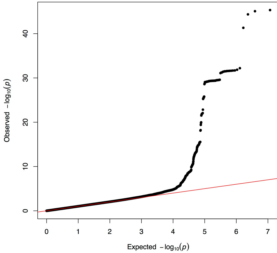
Supplementary Figure 3. QQ plot for genome wide analysis of cirrhosis. Lambda = 1.02
