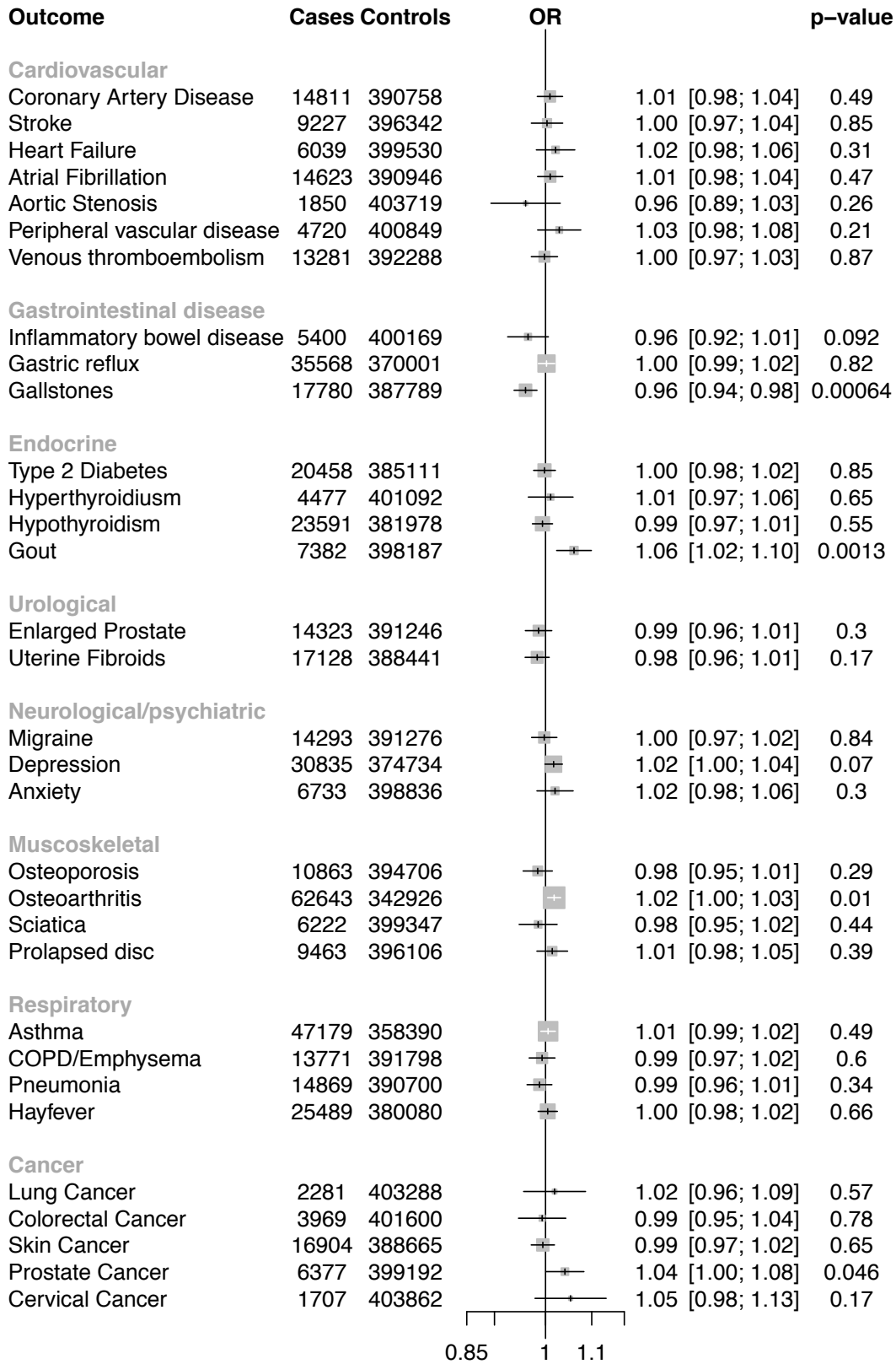
Supplementary Figure 6. Association of MARC A165T with other diseases in a phenome wide association study.
