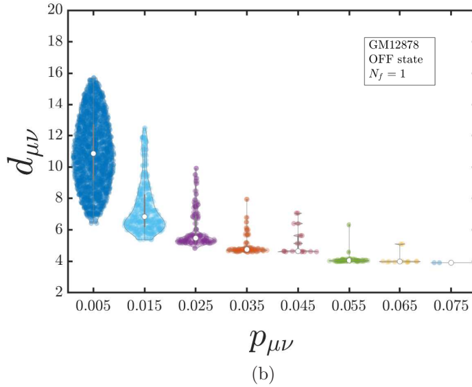
Figure S9: Violin plots showing the probability distribution of mean 3D distances for selected ranges of contact probabilities in (a) the K562 (ON state) cell lines, and (b) the GM12878 (OFF state) at normalization factor N_f = 1 .
