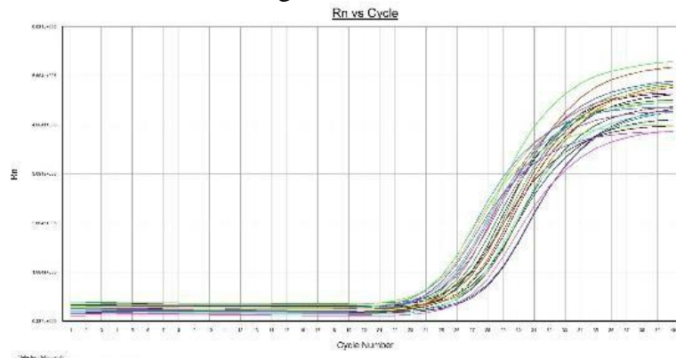
Figure 1 . RT-PCR curve. A: RT-PCR amplification curve of the FFAR2 gene; B: RT-PCR dissolution curve of the FFAR2 gene
