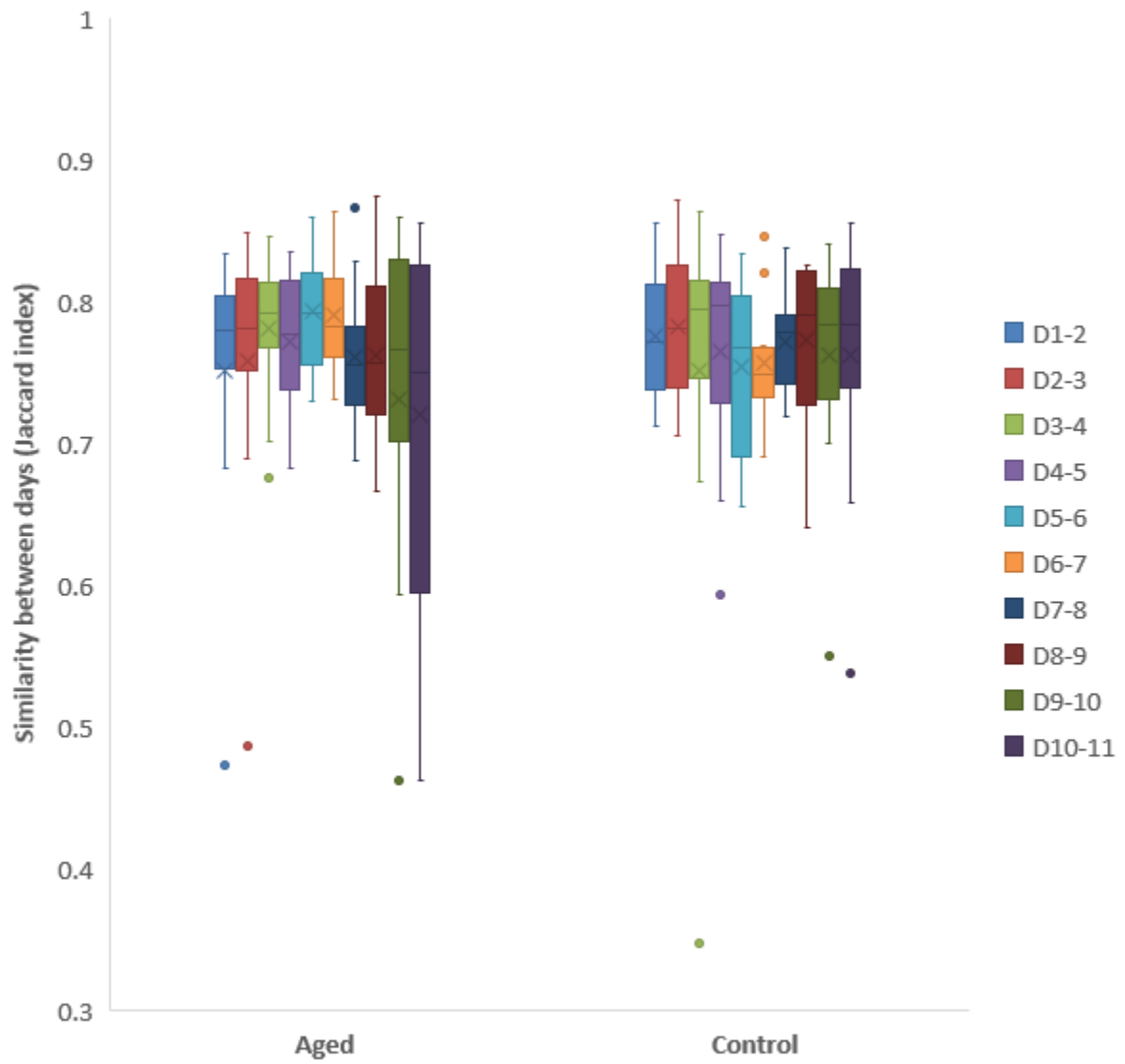
Figure S3: Jaccard index between the individual study days for the Control and Aged groups
