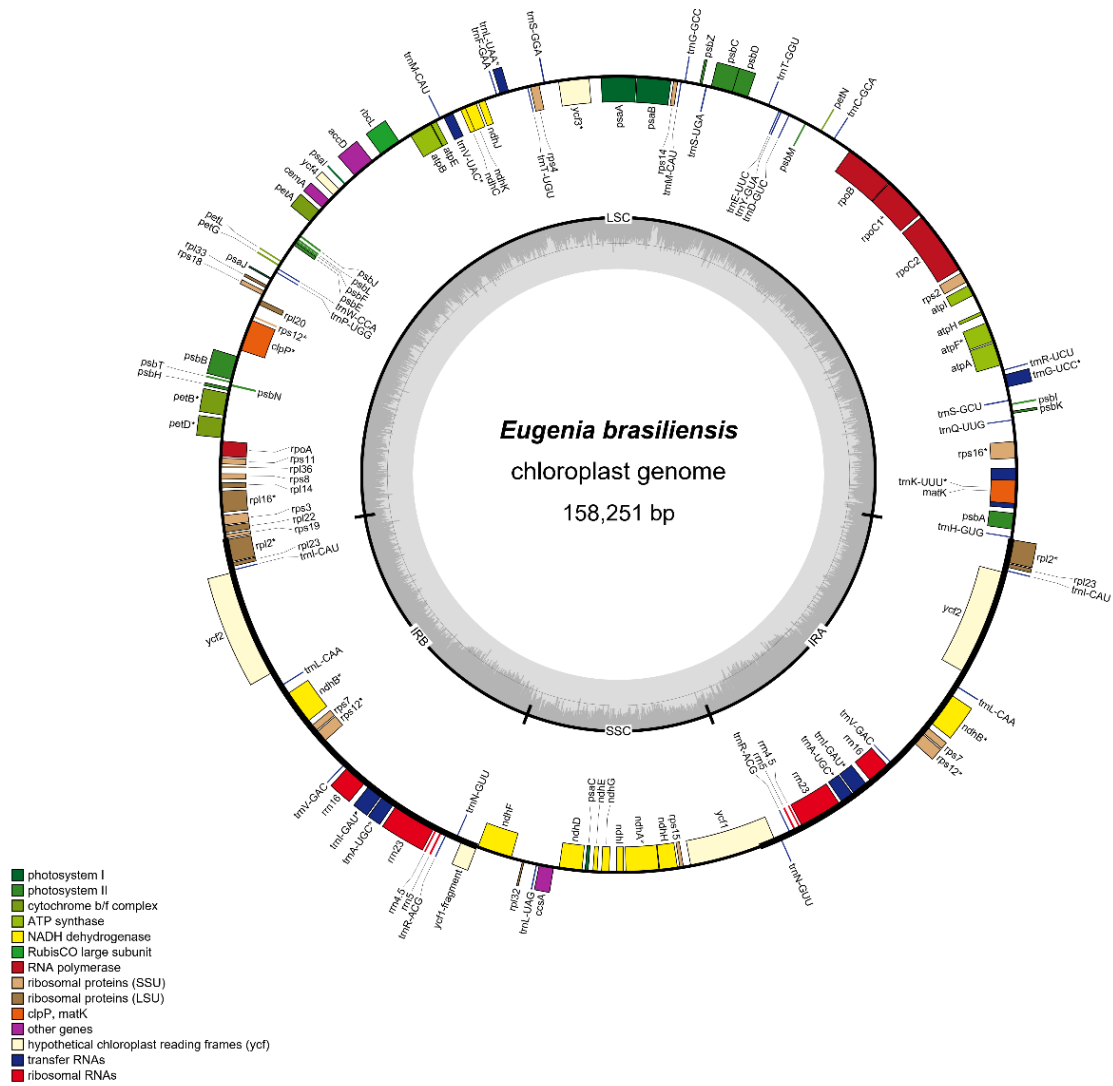
Figure S1 - Gene map of Eugenia brasiliensis chloroplast genome.
