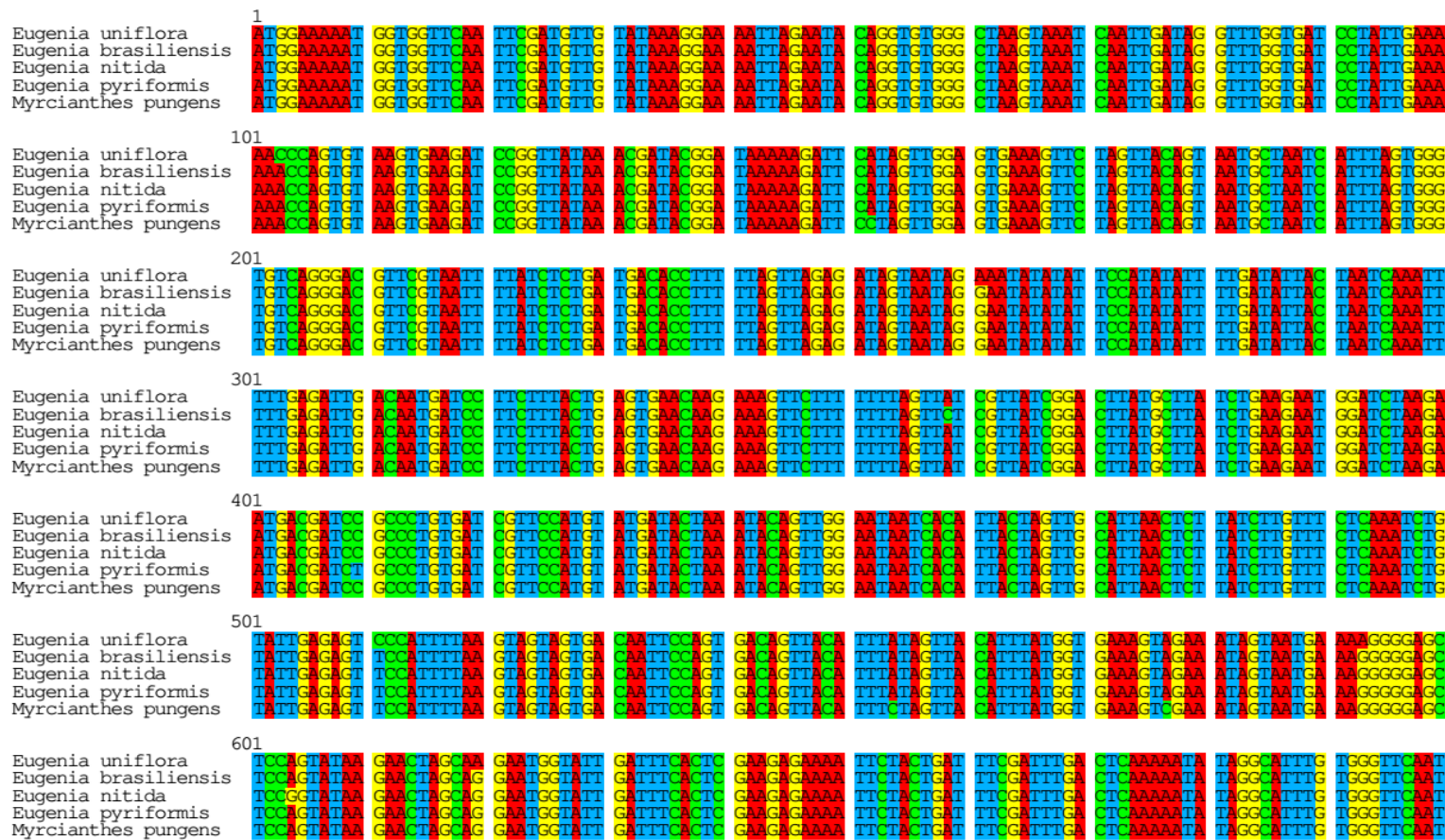
Figure S10 - Nucleotide alignment of accD , ccsA , rpoC2 , matK , ndhF and ycf1 .
