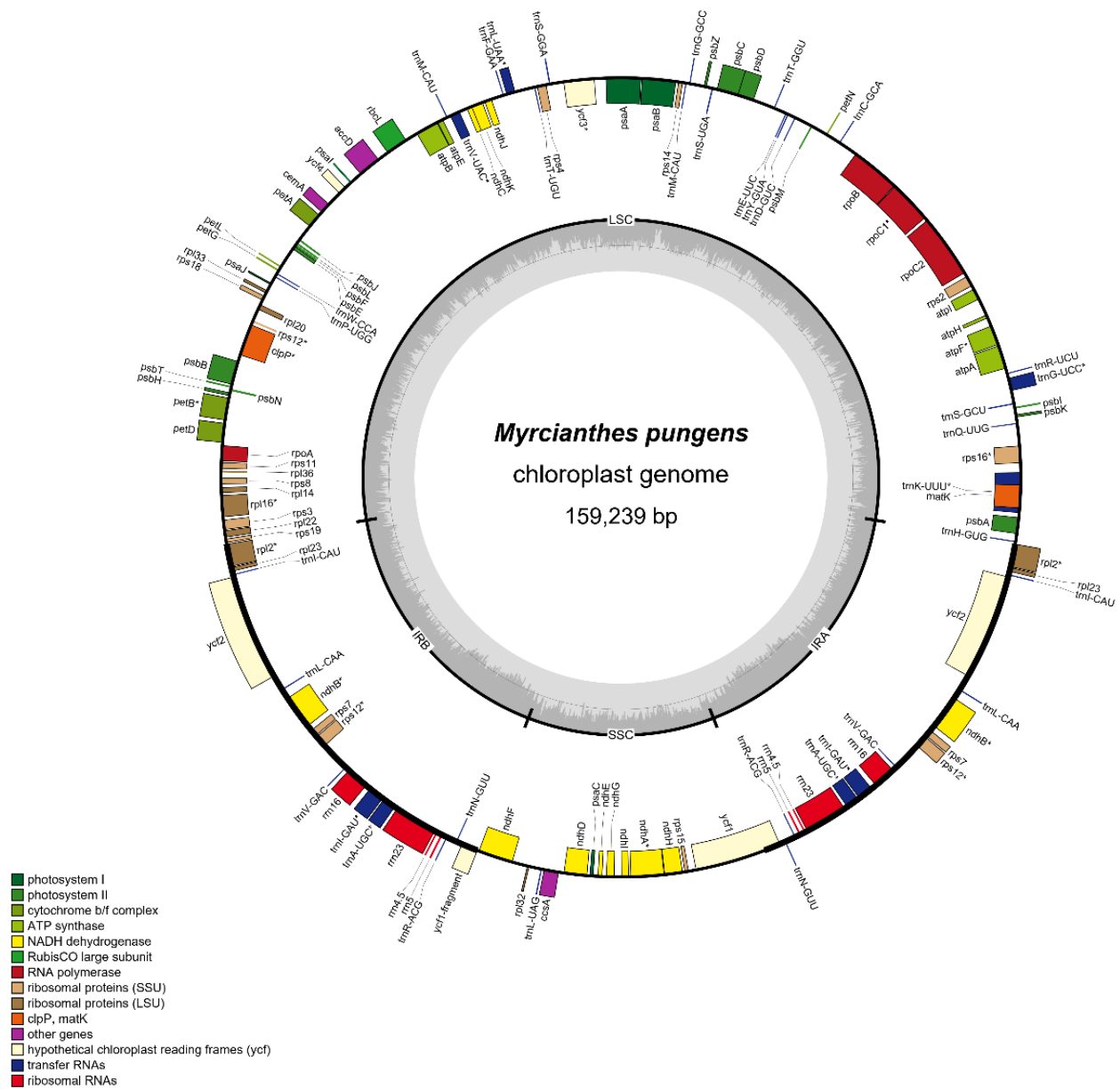
Figure S4 - Gene map of Myrcianthes pungens chloroplast genome.
