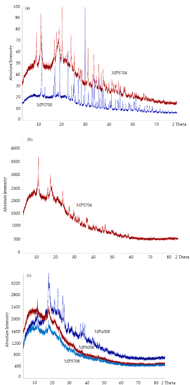
Figure S1. X-ray diffractograms of the chitosan microparticles: MP5700 and MP5704 (a), MP5706 (b), MP5708, MP5008 and MP4008 (c).
