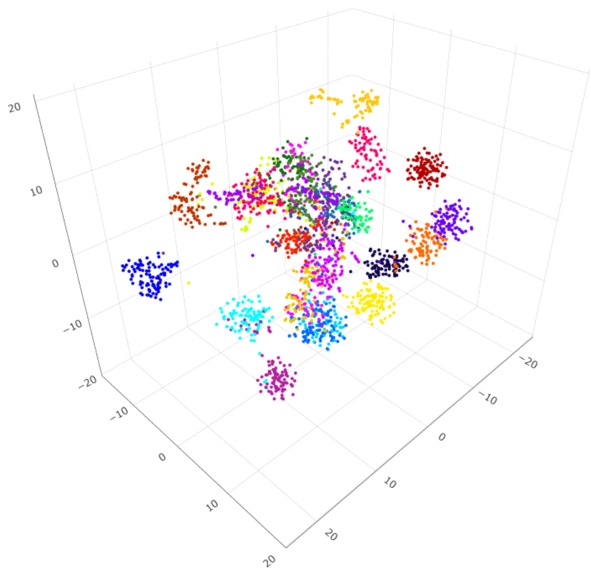
Original dataset
