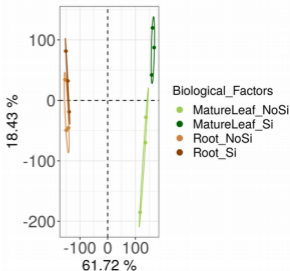
PCA on normalized counts
