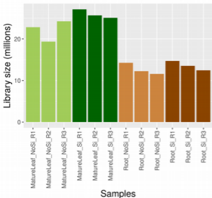
Total normalized counts per sample
