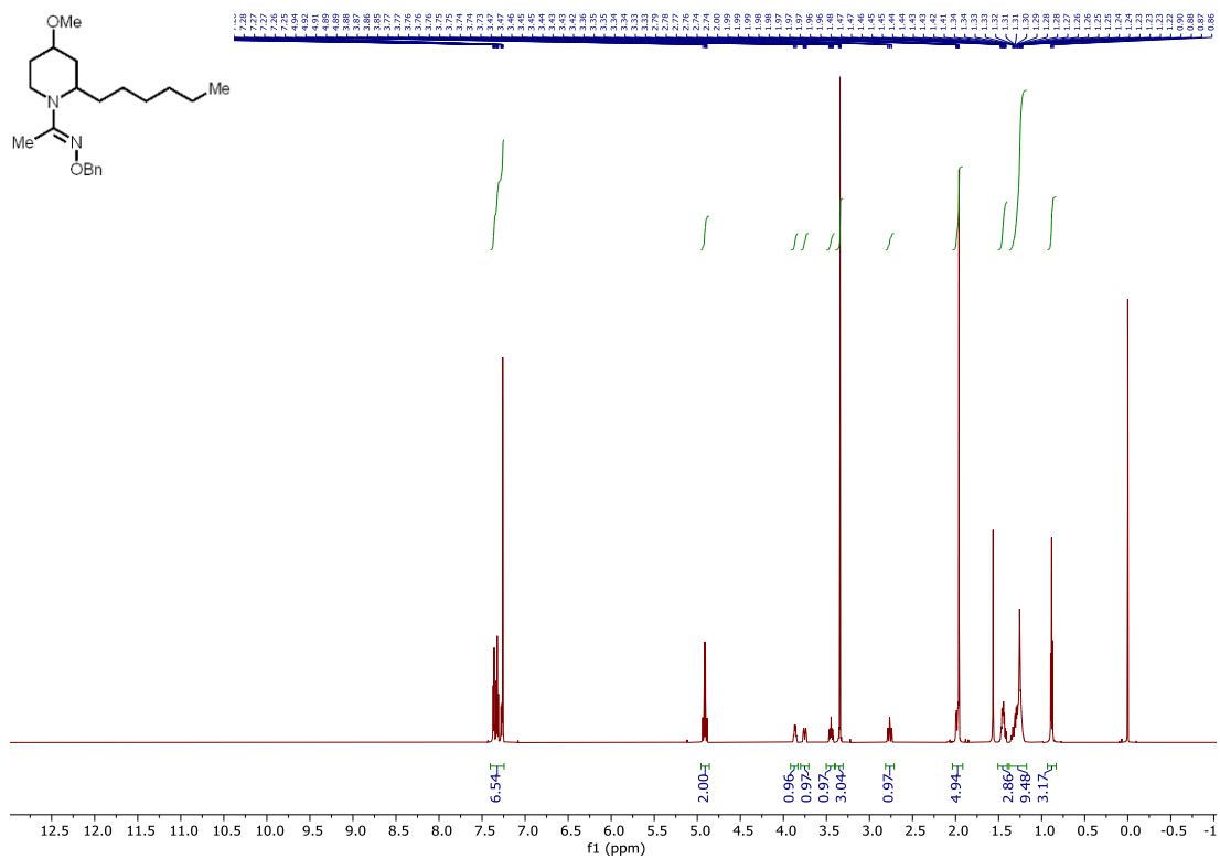
Second diastereomer
