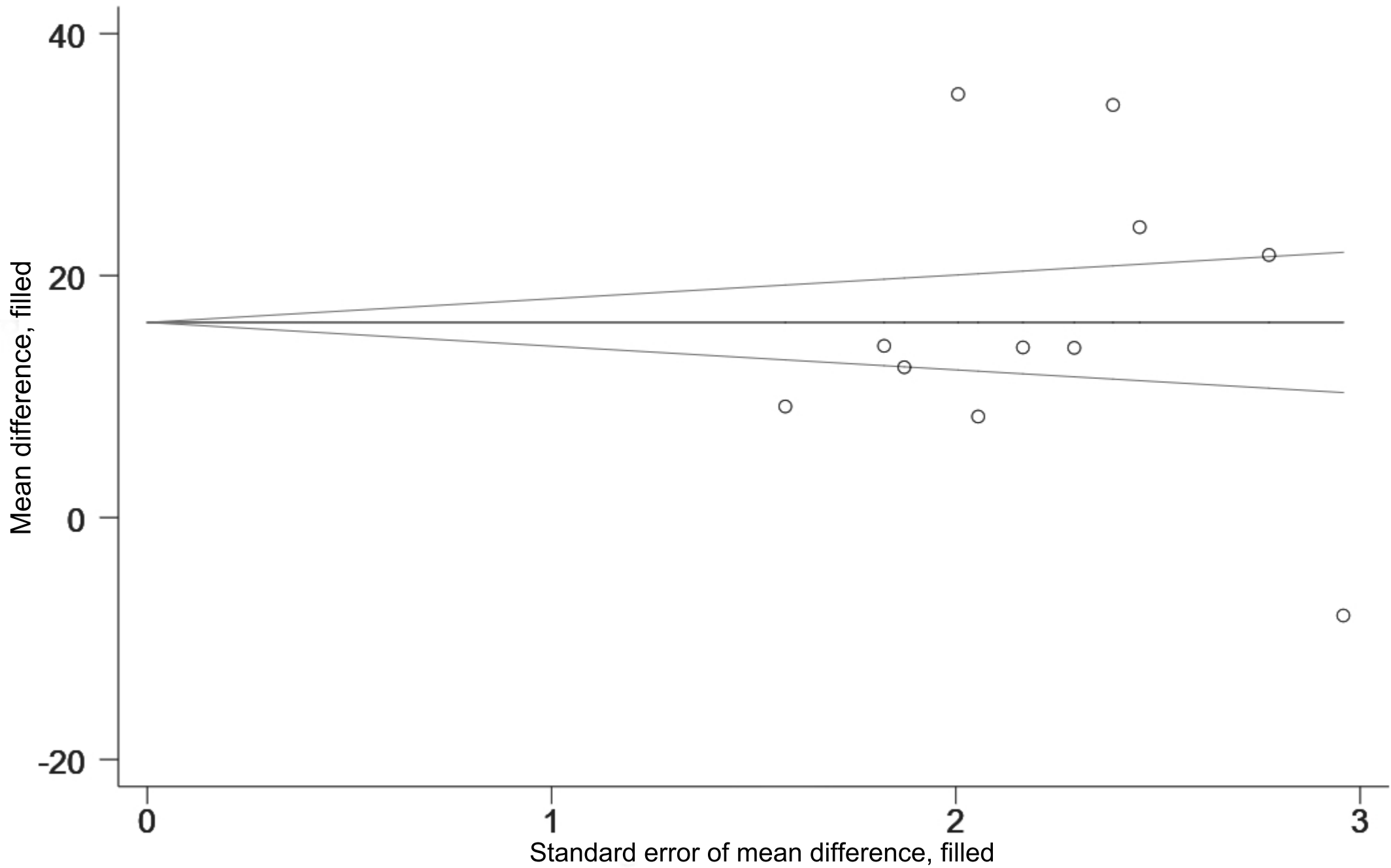
Fig. 9, Supplemental Digital Content. Filled funnel plot of serum ALT change in comparison of acupoint embedding alone or in combination versus conventional medications
