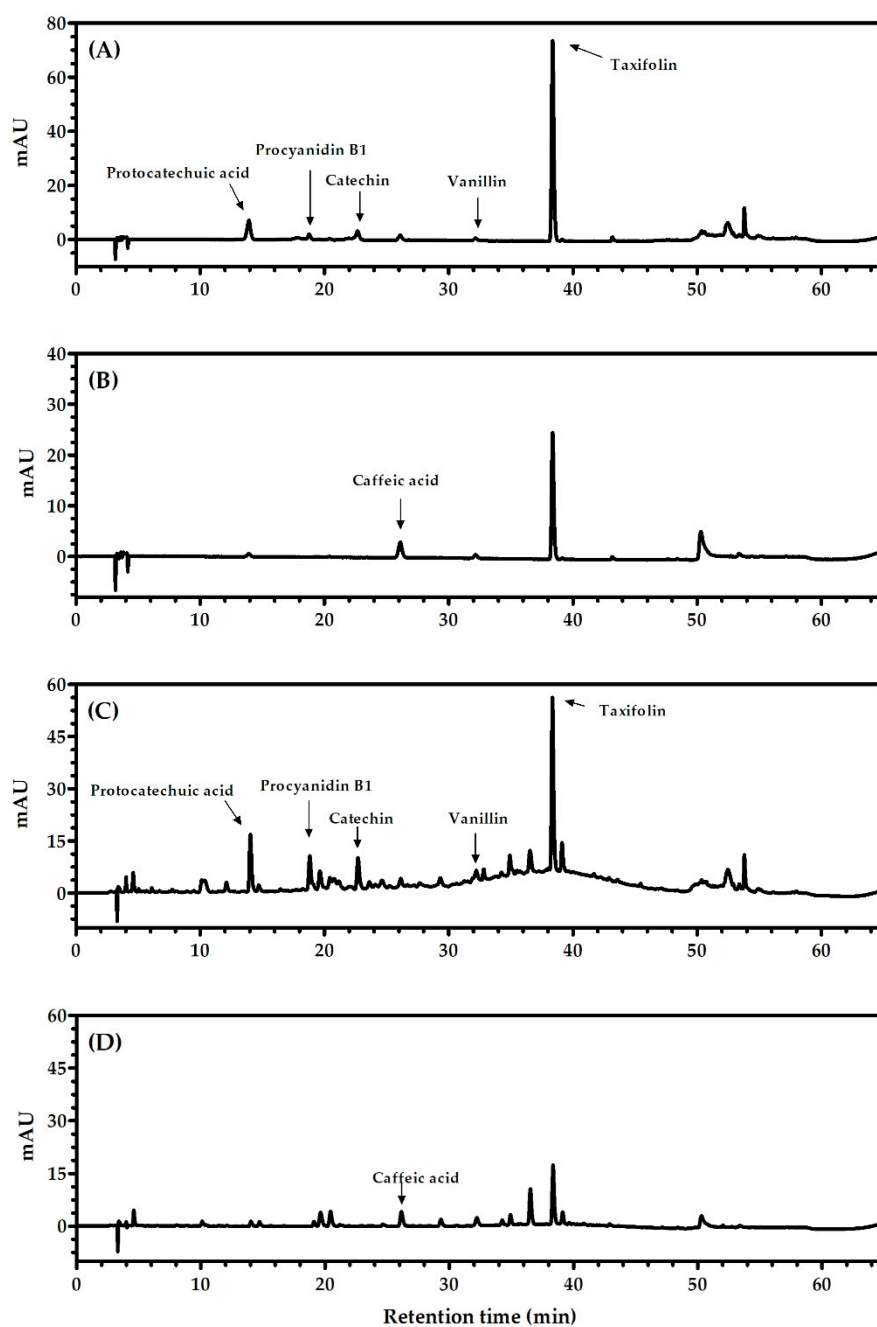
Supplementary Figure S1. High-performance liquid chromatography traces of mixture of standards at 280 nm (A) and 320 nm (B), and Korean red pine ( Pinus densiflora Sieb. et Zucc.) bark extract at 280 nm (C) and 320 nm (D).
