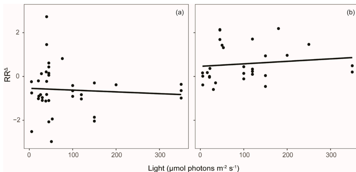
Figure S1. The natural log response ratios ( RR^A ) for toxin content plotted against irradiance for (a) N and (b) P limitation. (a) R^2=-0.02 , P=0.68 , (b) R^2=-0.03 , P=0.71 .
