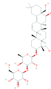
Saikosaponin B1
