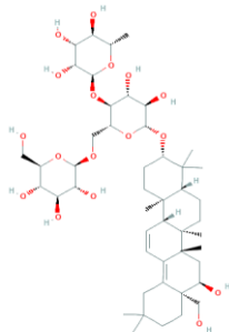
Saikosaponin BK1
