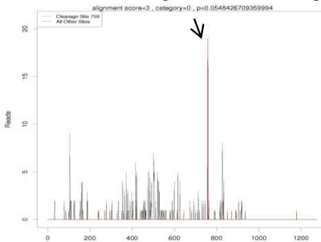
miR156e slicing JcSPL5 at 759 bp
