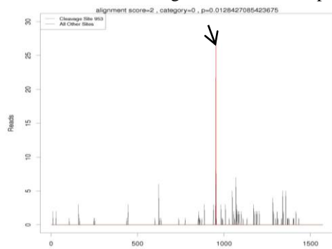
miR156a slicing JcSPL9 at 953 bp
