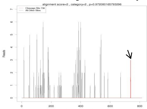
miR156d slicing JcSPL3 at 738 bp
