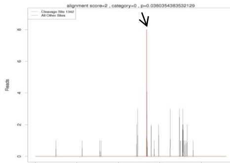
miR156f slicing JcSPL10 at 1342 bp
