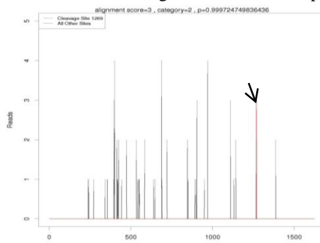
miR156a slicing JcSPL13 at 1269 bp
