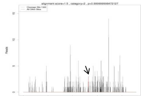
miR156d slicing JcSPL6 at 1320 bp
