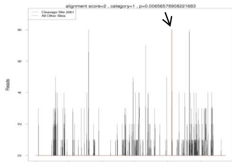
miR156a slicing JcSPL2 at 2061 bp
