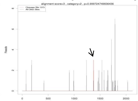
miR156a slicing JcSPL11 at 1373 bp
