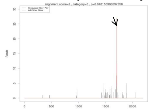
miR156a slicing JcSPL16 at 1707 bp
