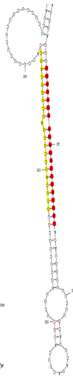
JcMIR156d
