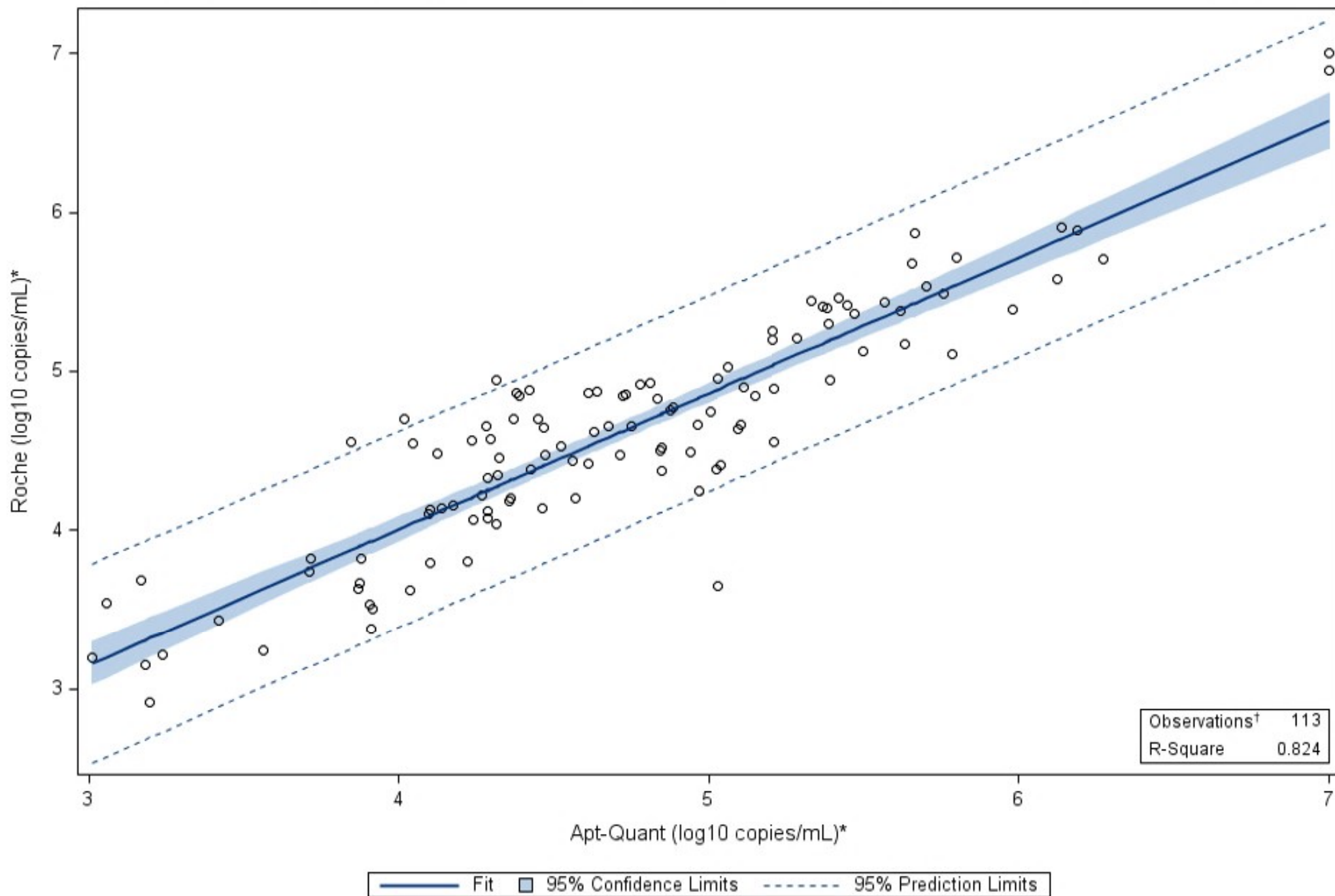
Supplemental Figure 2. Viral Loads Detected by the Roche COBAS AmpliPrep/COBAS TaqMan HIV-1 Test v2.0 and Hologic Aptima HIV-1 Quant Assay Among 113 Specimens with Reactive Antigen/Antibody Screening Results.
