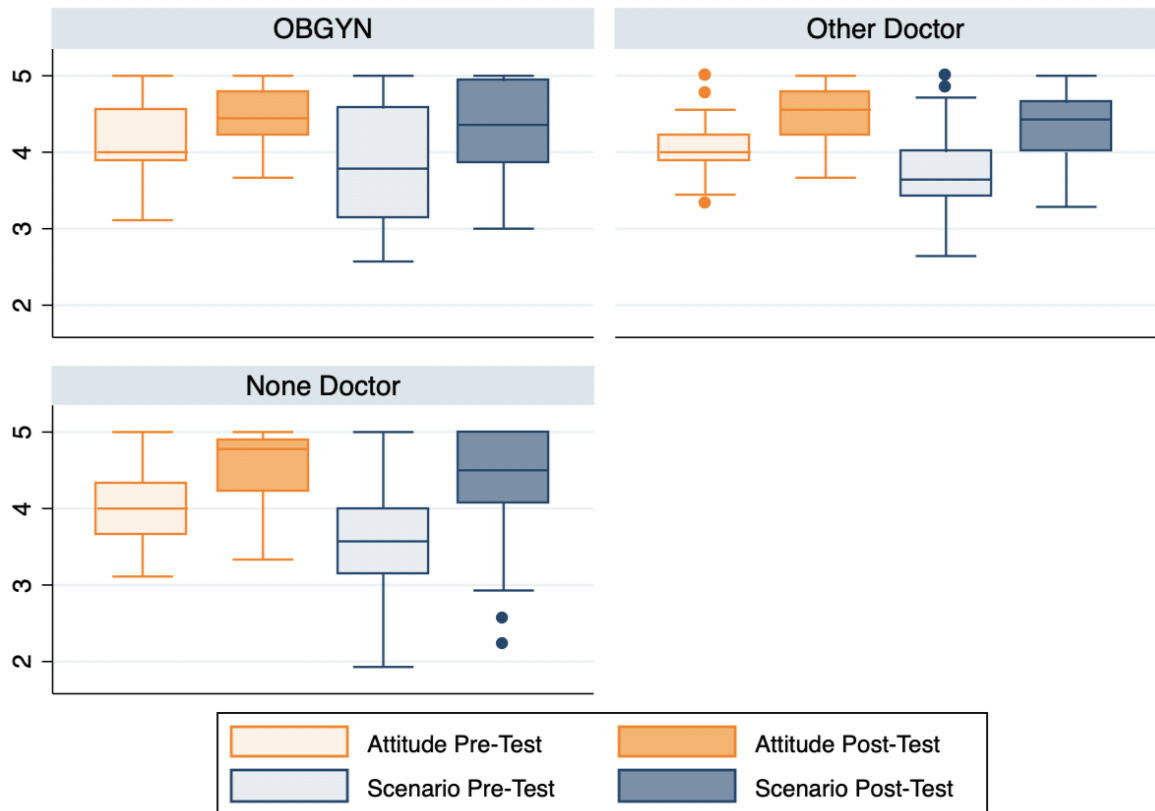
Figure S1. Box Plot of the Average Pre-test and Post-test Response by career type.
