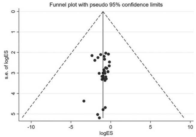
SUPPLEMENTARY FIG. S1. Funnel plot to assess for small study effects.
