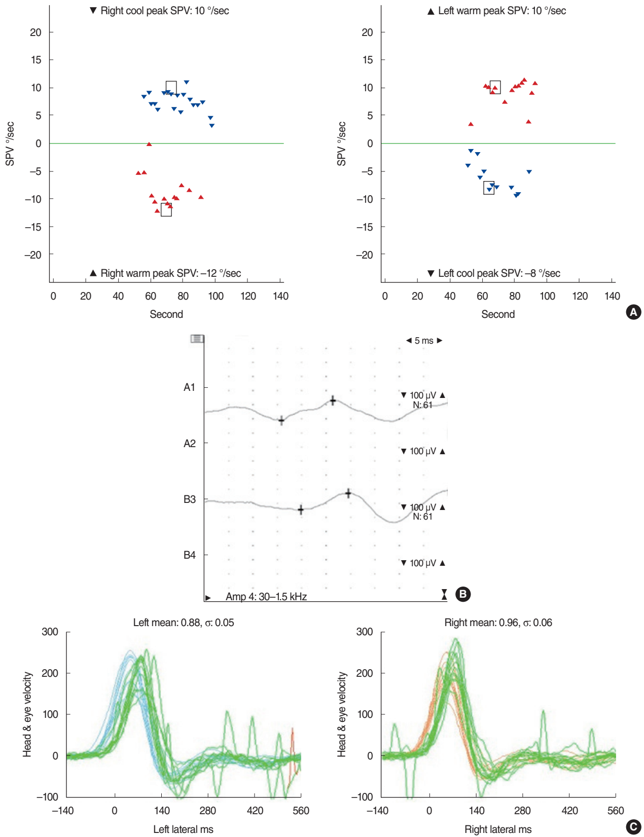
Supplementary Fig. 1. Comprehensive vestibular function test. (A) Bithermal caloric test. (B) Cervical vestibular-evoked myogenic potentials. (C) Video head impulse test. SPV, slow phase velocity.
