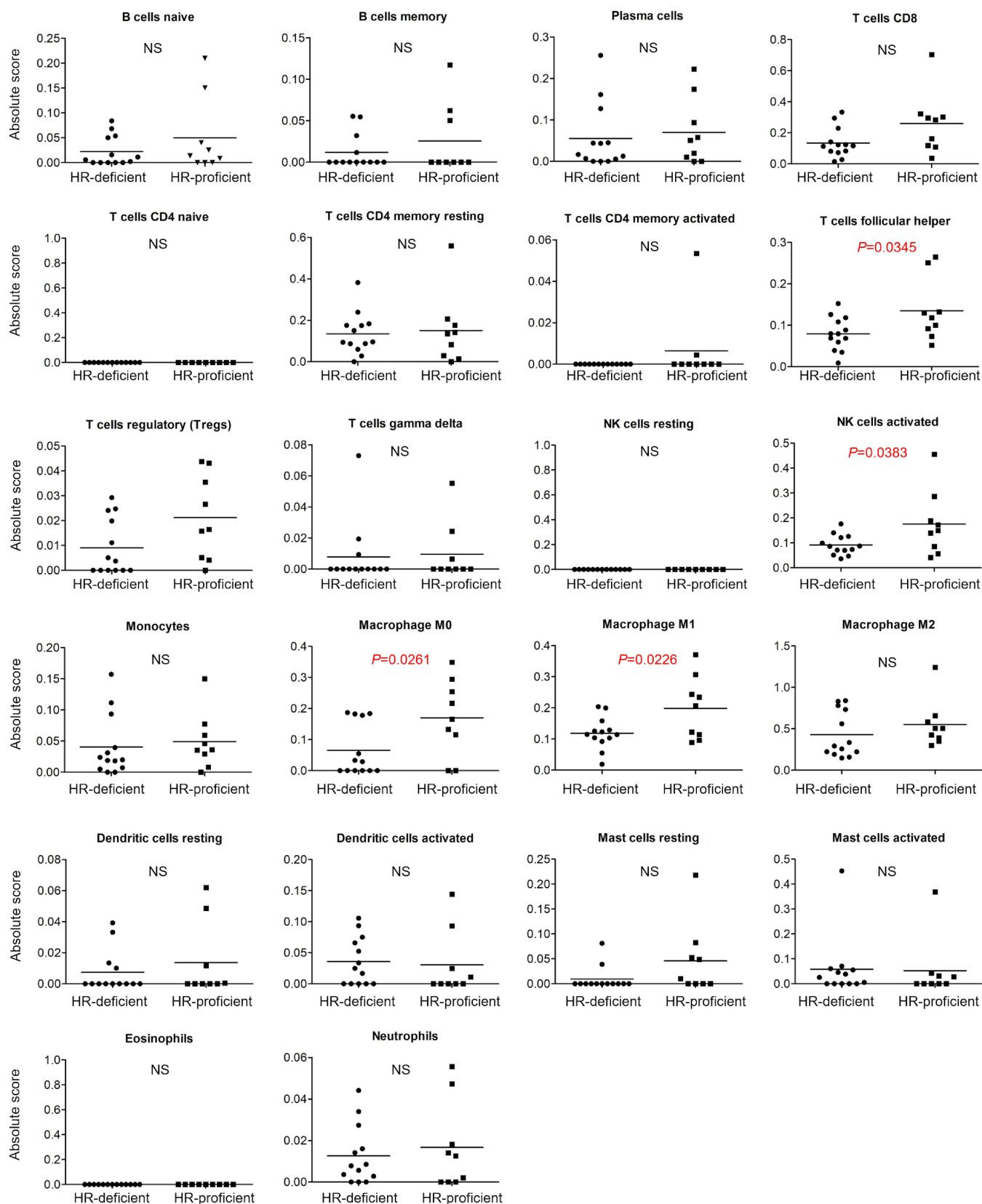
Supplementary figure S2. The absolute scores of each immune cell subtype in HR-proficient (n=9) and HR-deficient (n=13) tumors were shown. NS, not significant.
