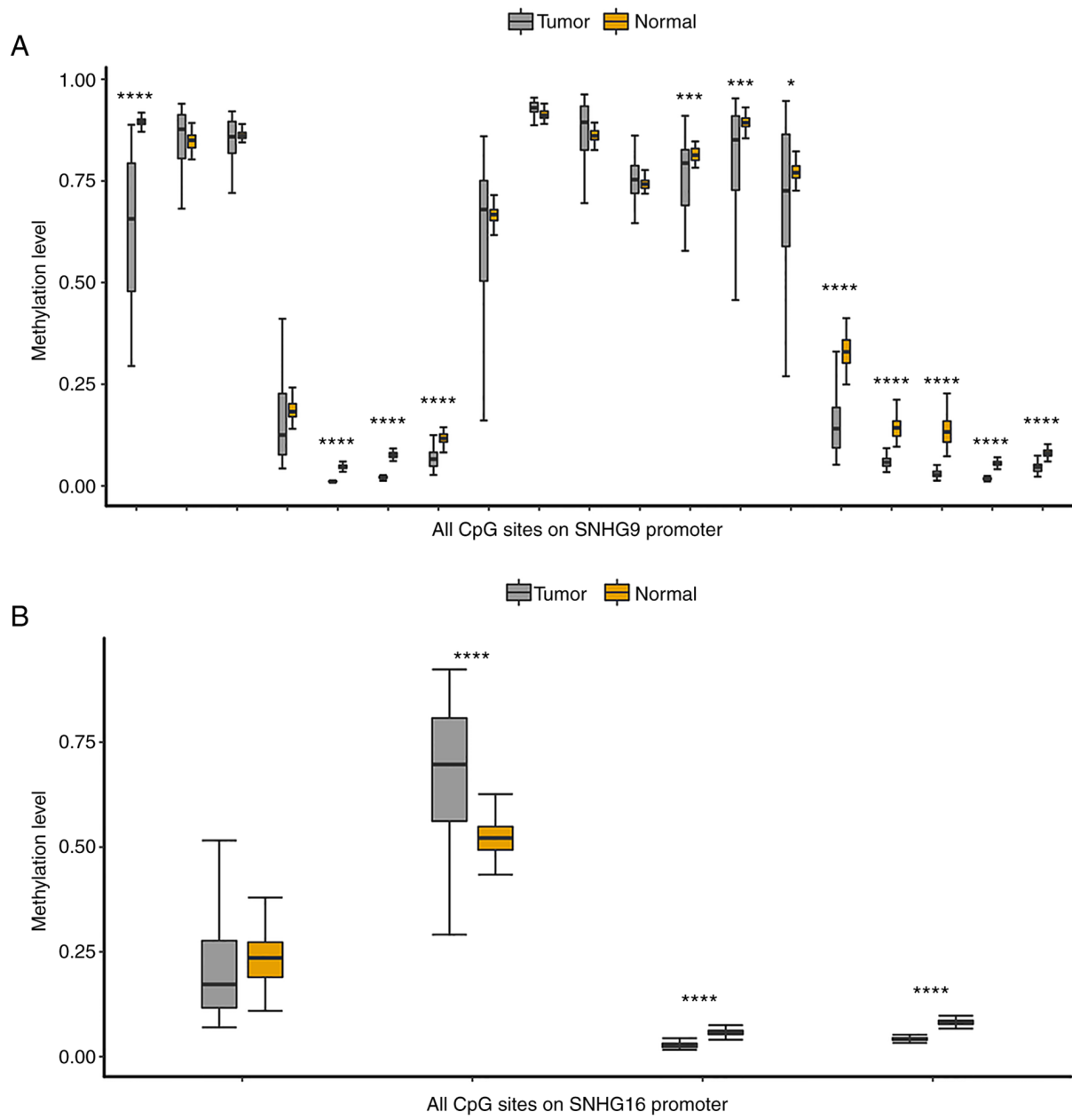
Figure S2. Boxplots with comparisons of methylation levels between glioblastoma and normal samples of all CpG probes annotated to the SNHG9 promoter and the SNHG16 promoter. The probe sequences closer to the right in the figure were closer to the transcriptional start site. * P \leq 0.05 , ** P \leq 0.001 , *** P \leq 0.0001 vs. respective tumor tissue. SNHG, small nucleolar RNA host gene.
