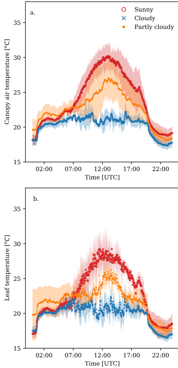
Figure S6: (a) Canopy air temperature and (b) leaf temperature. Bold lines represent the average value, whereas the shaded area represents the standard deviation over the days for sunny (red), cloudy (blue) and partly cloudy days (orange).
