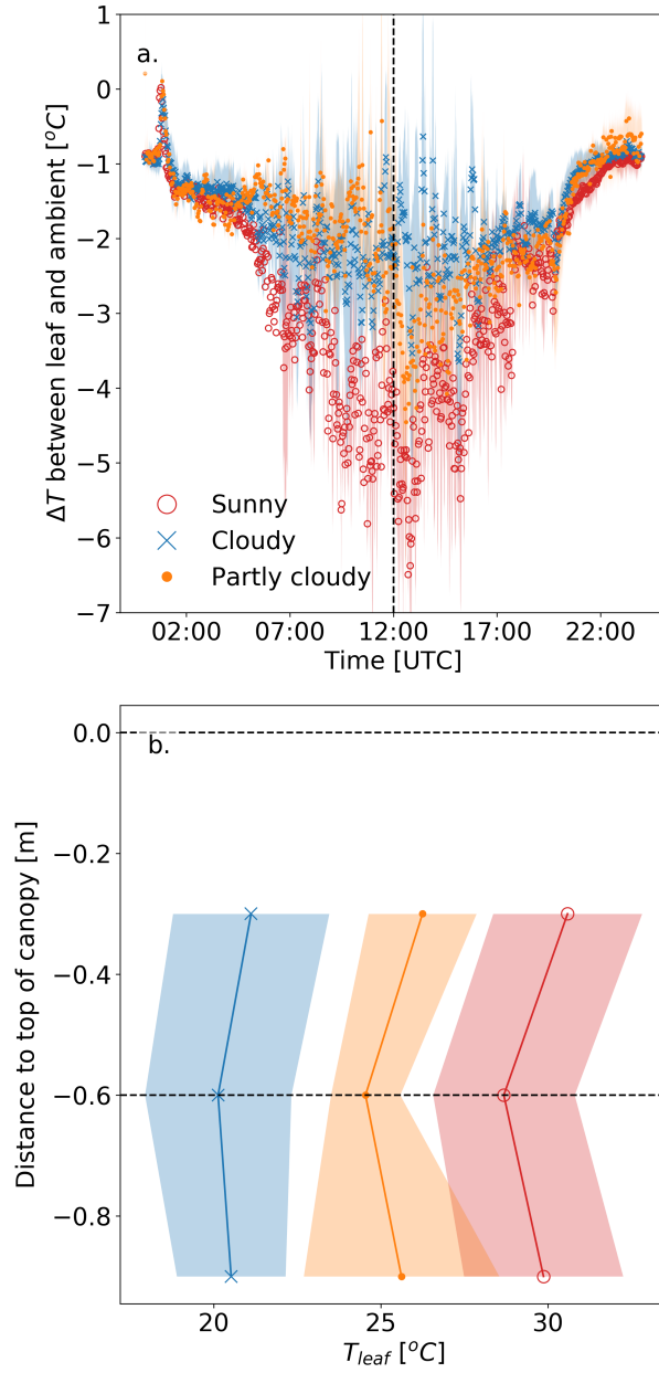
Figure S7: Difference between leaf temperature (at 60 cm below the top of the canopy) and ambient temperature. Bold lines represent the average value, whereas the shaded area represents the standard deviation over the days for sunny (red), cloudy (blue) and partly cloudy days (orange). a.) time course of the temperature difference, where the dashed line indicates noon. (b) vertical leaf temperature profile in the canopy at noon; the dashed lines show the heights at which the differences between leaf and ambient temperature were calculated.
