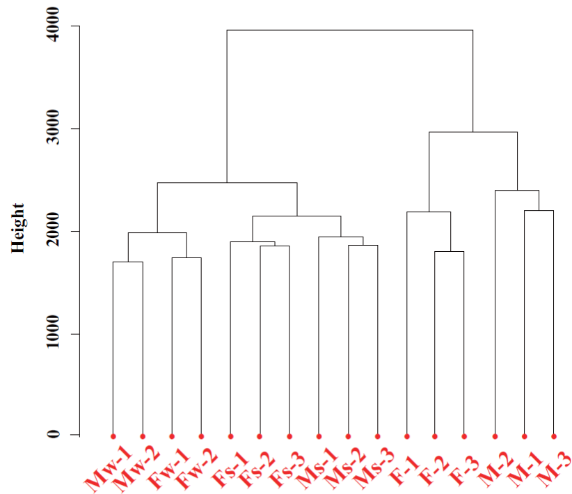
Samples Distance method: "euclidean"; Clustering method: "ward"
