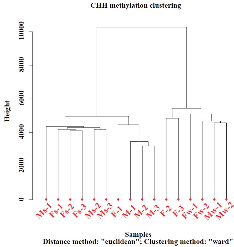
Supplementary Figure 1 Hierarchical clustering of 16 samples in CpG, CHG and CHH contexts
