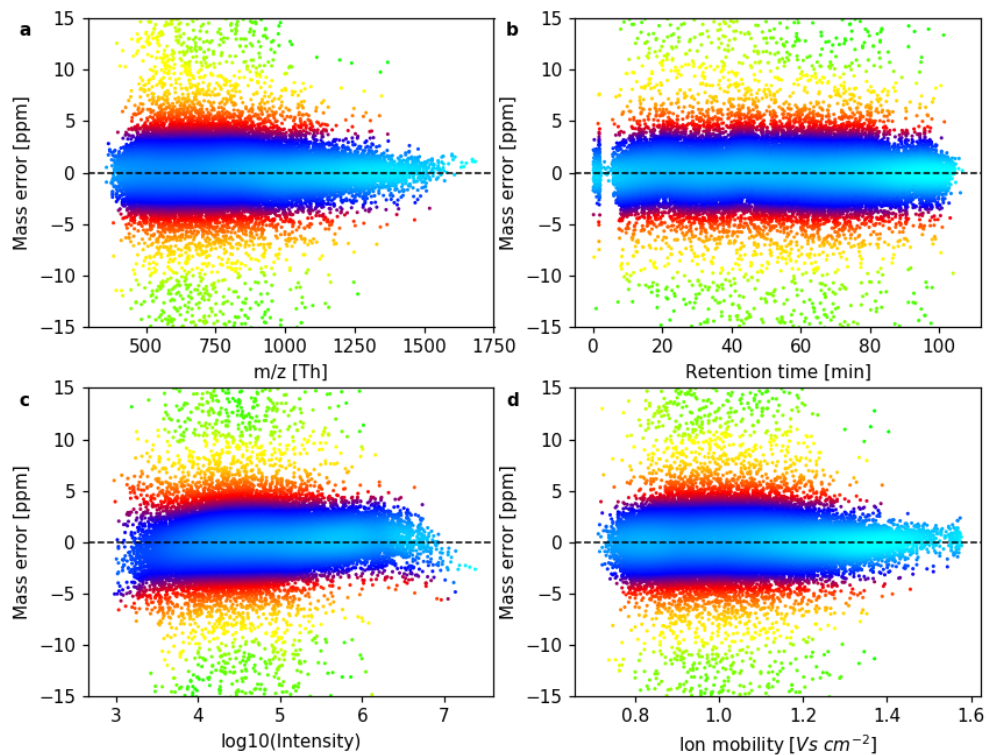
Supplementary Figure 1. Mass error after recalibration. a.-d. Residual mass errors after complete recalibration, showing the dependence of the residual mass error on m/z ( a. ), retention time ( b. ), logarithm of the peak intensity ( c. ) and ion mobility ( d. ). Colors reflect the density of data points.
