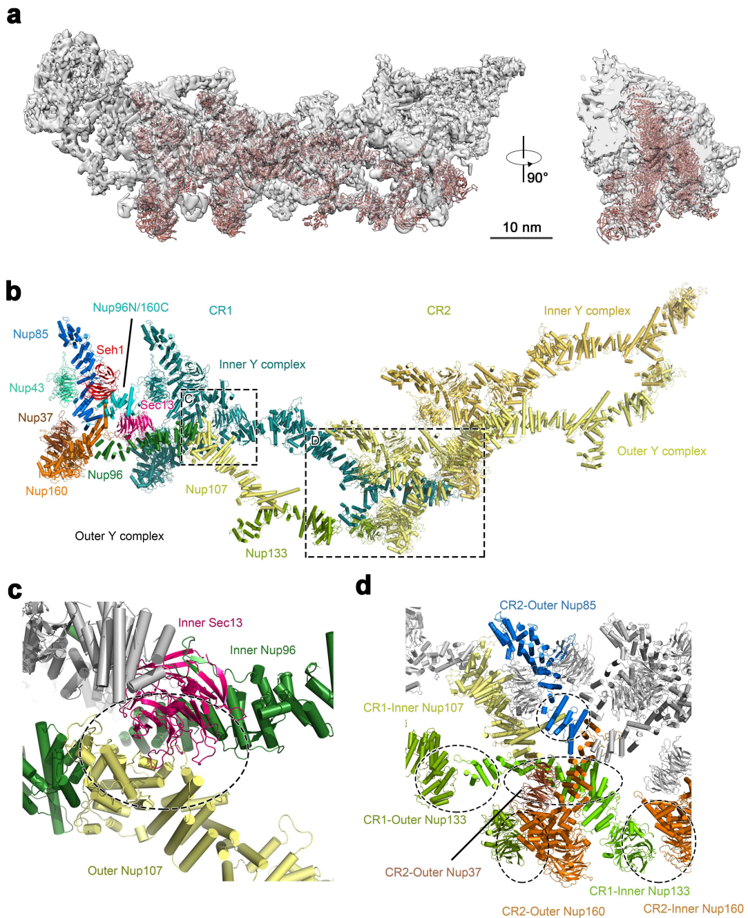
Supplementary information, Fig. S10 | Interactions among the Y complexes. a , The final coordinates of the inner and outer Y complexes are placed into the EM density map. Two views are shown. b , Interactions among the Y complexes within the same CR subunit and between two adjacent subunits. The inner and outer Y complexes interact with each other within the same subunit. A pair of Y complex from one subunit associate with its counterpart from the adjacent subunit in a head-to-tail fashion. c , A close-up view on the interface between the inner and outer Y complexes within the
