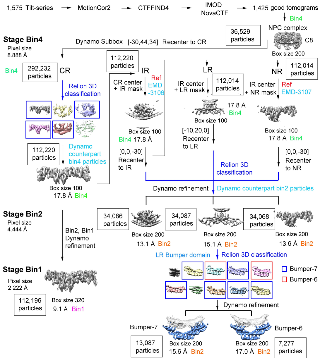
Supplementary information, Fig. S2 | A processing flow chart of the cryo-ET data on the NPC from Xenopus laevis ( X. laevis ). For detailed description, please refer to the Methods. CR, cytoplasmic ring; IR, inner ring; LR, luminal ring; NR, nuclear ring.
