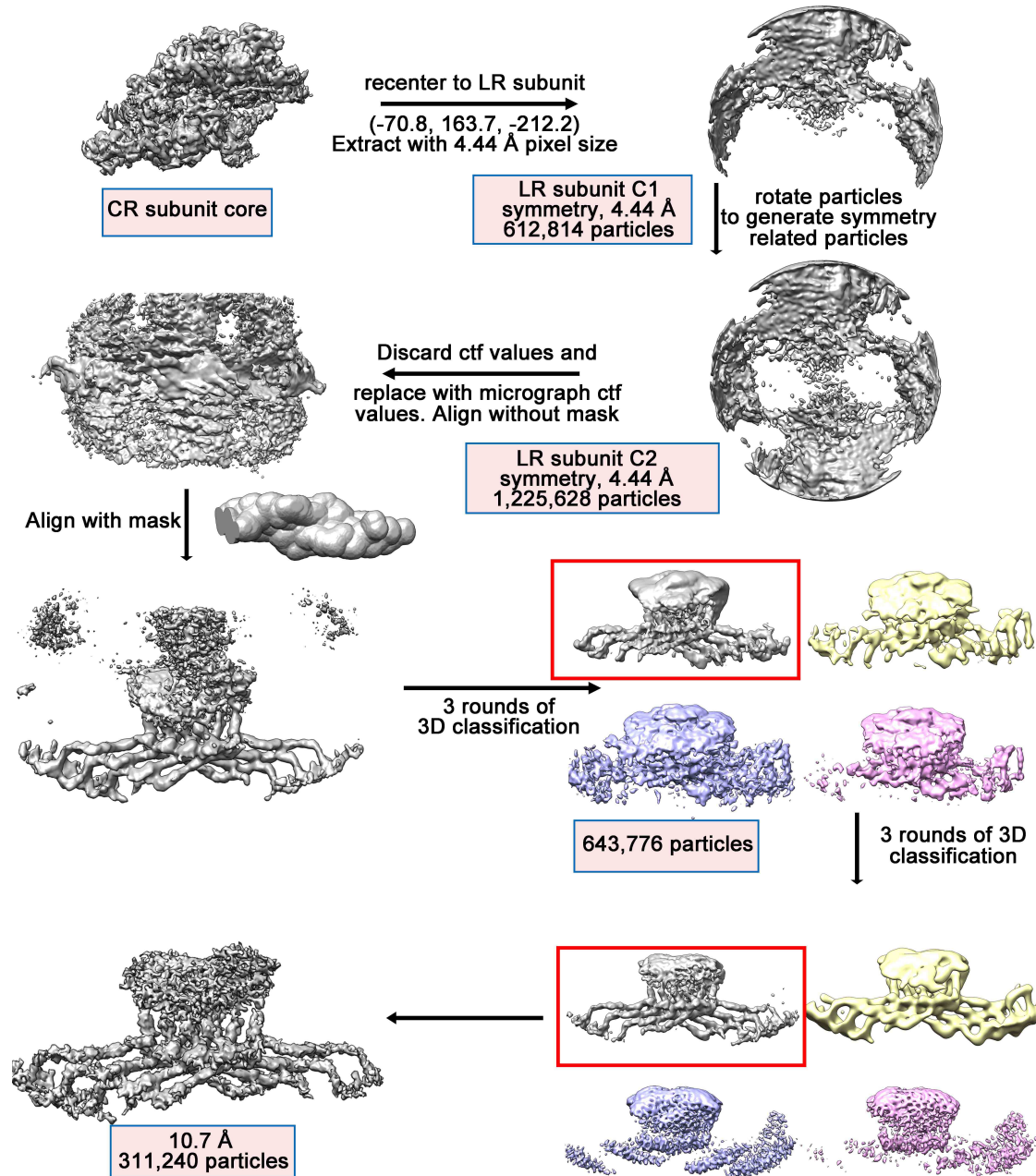
Supplementary information, Fig. S5 | A flow chart for the processing of the cryo-EM data on the LR subunit of the NPC from X. laevis . Single-particle analysis (SPA) was applied in data processing. For detailed description, please refer to the Methods.
