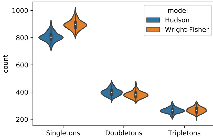
S1 Figure. Number of singletons, doubletons, and tripletons simulated under Wright-Fisher and Hudson coalescent models. A 1Mb region was simulated 100 times in 20,000 haploid lineages in a diploid population of 10,000 individuals.
