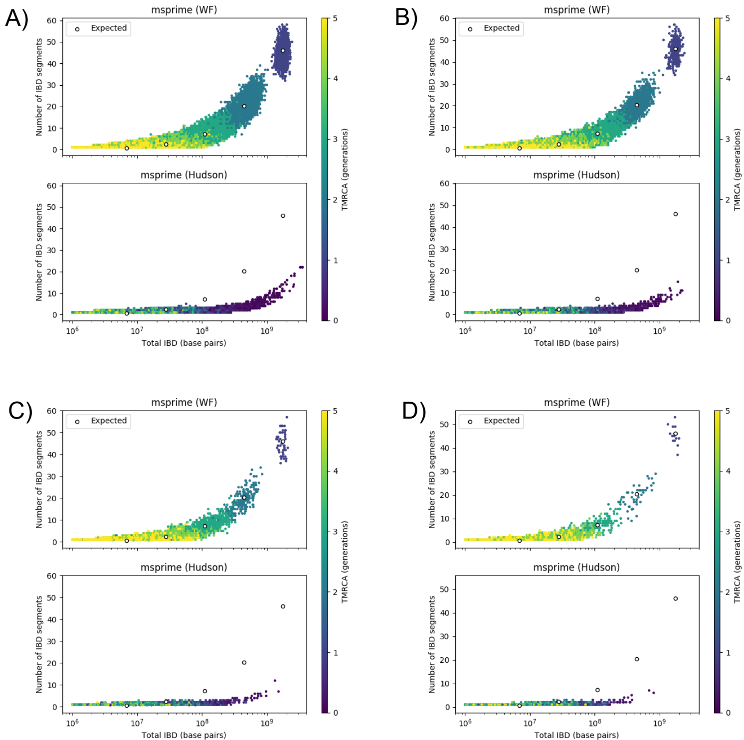
S3 Figure. Number of IBD segments between pairs of individuals versus total length of shared IBD segments. 22 chromosomes of realistic lengths, simulated under Wright-Fisher model (top) and coalescent (bottom), compared to the analytical expectation under Eqs (1) and (2) of S3 Appendix. Effective population size 10,000, sample size A) 5000, B) 2500, C) 1000, D) 500. Minimum IBD segment length of 1 centimorgan.
