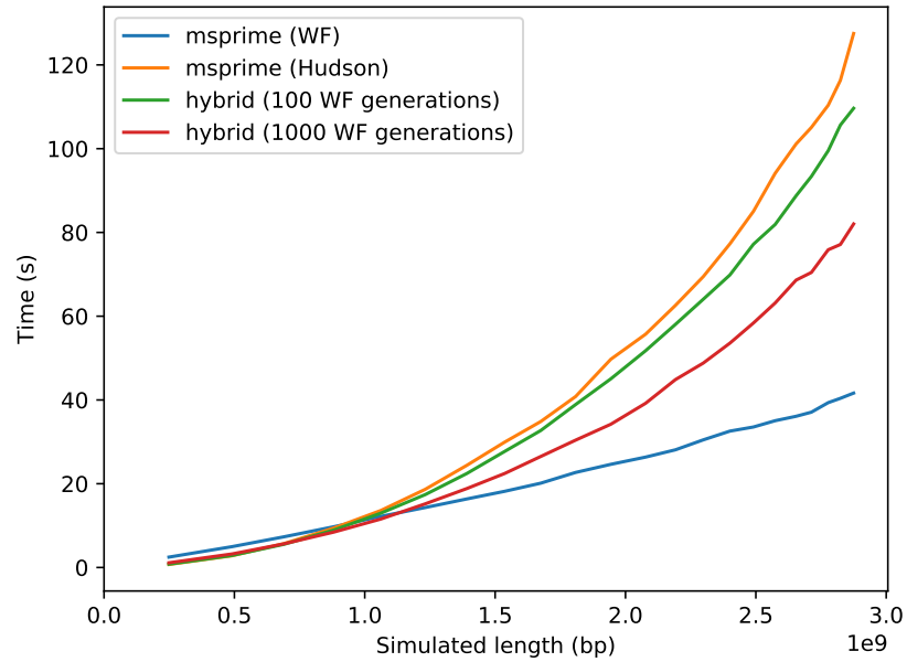
S5 Figure. Computation time of Hudson coalescent, Wright-Fisher, and hybrid models with 100 and 1000 Wright-Fisher generations before switching to the coalescent. Simulations contain from 1 to 22 chromosomes of realistic lengths, using the method described in S1 Appendix, in 500 haploid samples within a diploid population of size 500.
