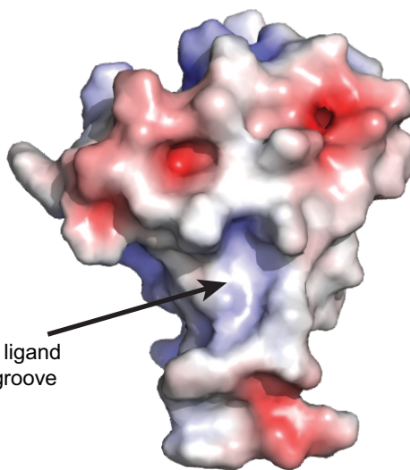
Surface view of ORF8-Ig domain
