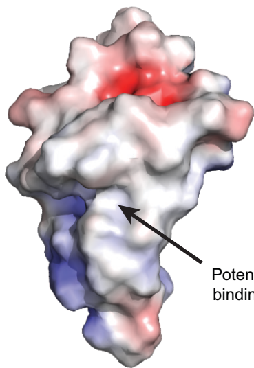
Surface view of ORF7a-Ig domain (PDB: 1xak_A)
