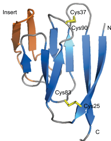
Model of ORF8-Ig domain
