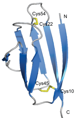
ORF7a-Ig domain (PDB: 1xak_A)
