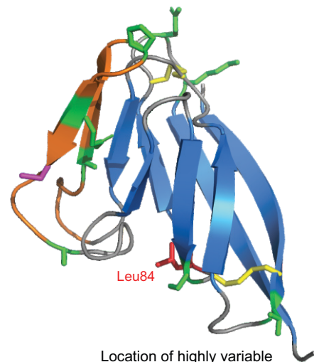
Location of highly variable residues of ORF8-Ig domain (sticks in green and red )
