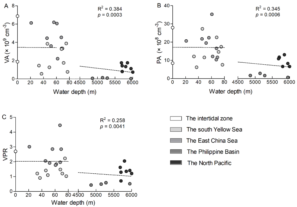
Figure S1. Spatial patterns of sediment (A) VA, (B) PA and (C) VPR along with the water depth gradient in the surveyed areas.
