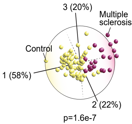
S7 Figure. Principal component analysis and hierarchical clustering heatmap analysis of multiple sclerosis (MS) blood miRNA expression profiles (GSE31568) shows that three circulating miRNAs, associated with inflammation and immune function, can identify the majority of MS patients.
