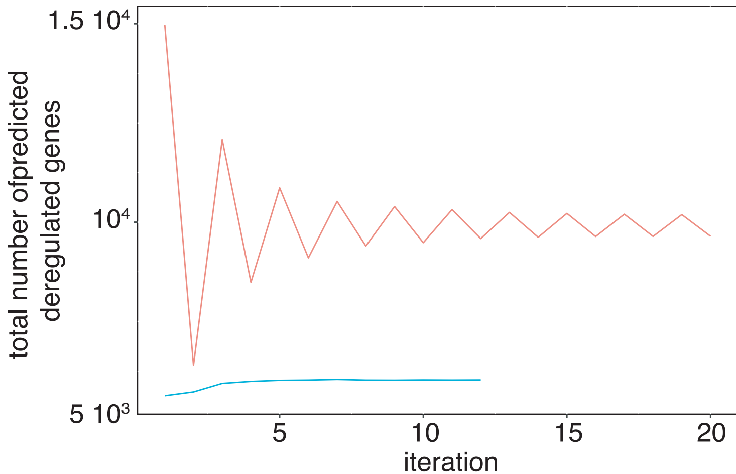
S1 Fig. Convergence towards a consistent list of deregulated genes is rapidly achieved by the PenDA method. We plotted the evolution of the total number of predicted deregulated genes during the successive iterations of the PenDA method applied to one simulated dataset with l=30 and h=0.1 (red line) or h=0.4 (cyan line).
