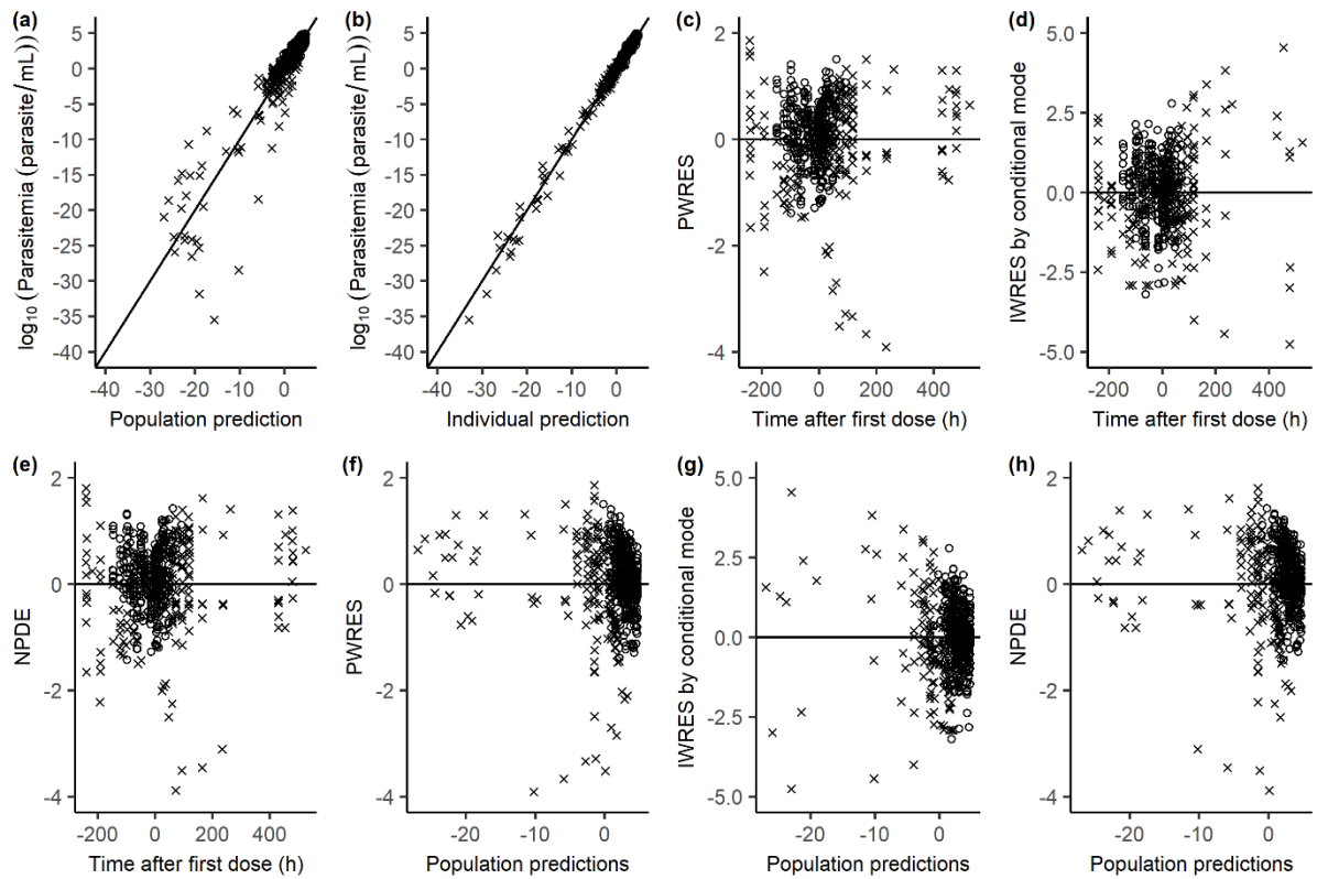
Figure S7 Goodness of fit plots of the final population pharmacodynamic model for P. vivax parasitemia for chloroquine whole blood data. The circles represent the data above the lower limit of quantification and the crosses represent the simulated values below the lower limit of quantification data. PWRES, population weighted residuals; IWRES, individual weighted residuals; NPDE, normalized prediction distribution errors.
