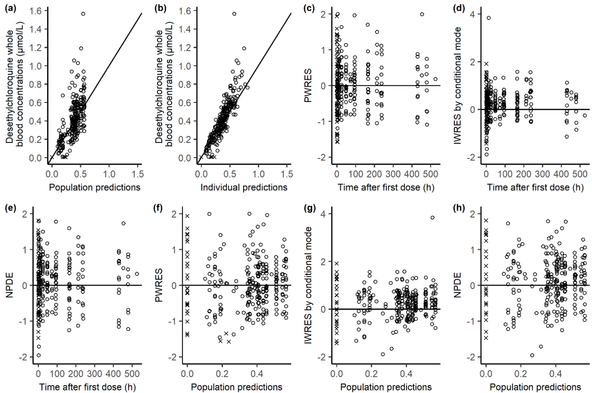
Figure S5 Goodness of fit plots of the final population pharmacokinetic model for desethylchloroquine whole blood concentrations. The circles represent the data above the lower limit of quantification and the crosses represent the simulated values below the lower limit of quantification data. PWRES, population weighted residuals; IWRES, individual weighted residuals; NPDE, normalized prediction distribution errors.
