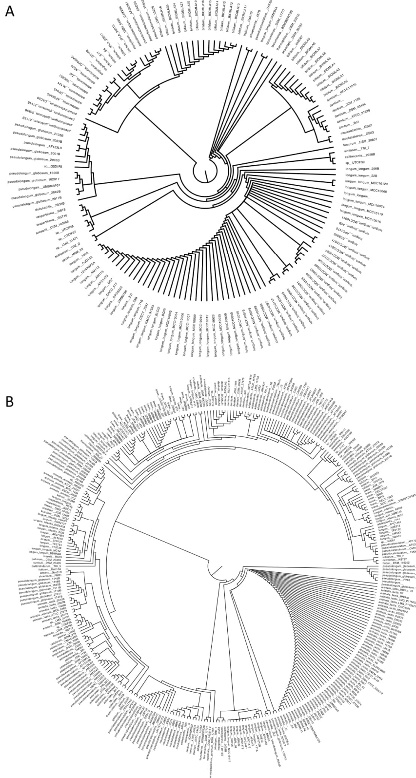
Figure S1: Phylogenetic analyses based on the amino acid sequences of (A) Cas 9 protein and (B) Cas3 protein in Bifidobacterium , with taxa names shown. The amino acid sequences were aligned using the MUSCLE alignment algorithm to generate neighbor-joining consensus trees based on the Jukes-Cantor model.
