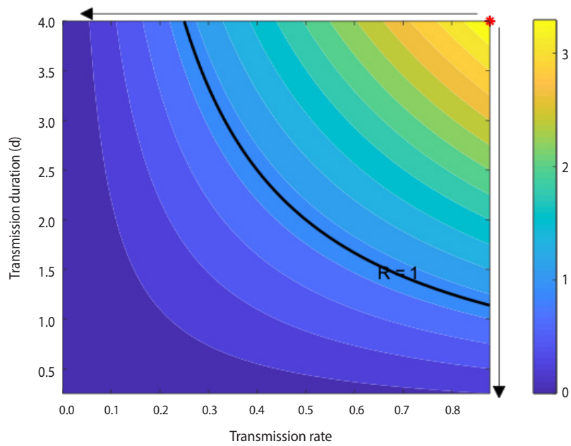
Appendix 1. A contour map of the reproductive number ( R ) as transmission rate and transmission duration changes. R=3.5 (red spot) and R=1 (black line).
