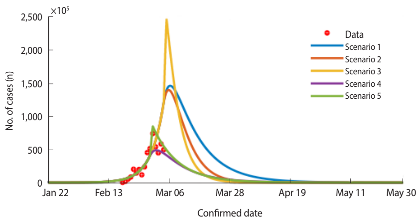
Appendix 3. Estimated daily number of confirmed patients by scenario in Daegu and North Gyeongsang Province. See Table 2 for scenarios. Number of cases (red dots) and model fitting curves (colored lines).
