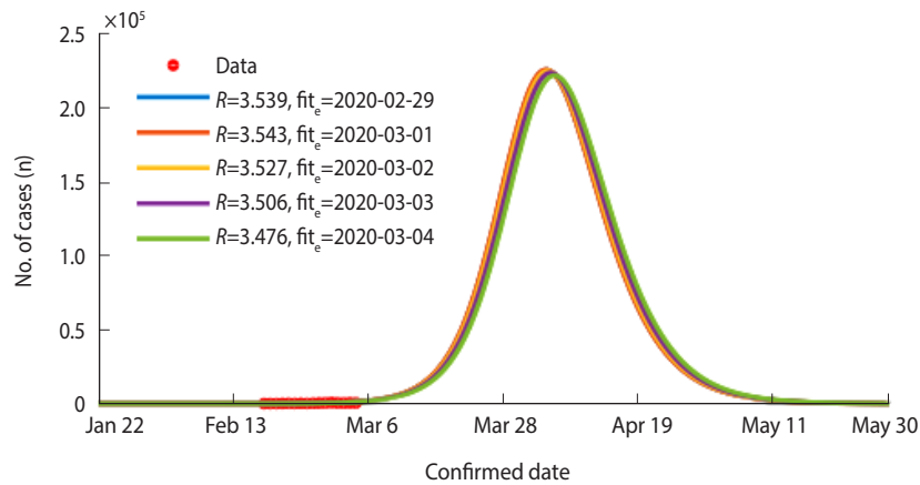
Appendix 2. Estimated reproductive number ( R ) and daily number of confirmed patients in Daegu and North Gyeongsang Province at base scenario which means no preventive measures. R varies with fitting period. Number of cases (red dots) and model fitting curves (colored lines).
