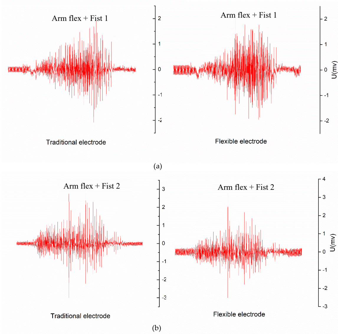
Figure S3. movements of arm flex combining fist (a) the sEMG of arm flex combining with fist 1 (b) the sEMG of arm flex combining with fist 2.
