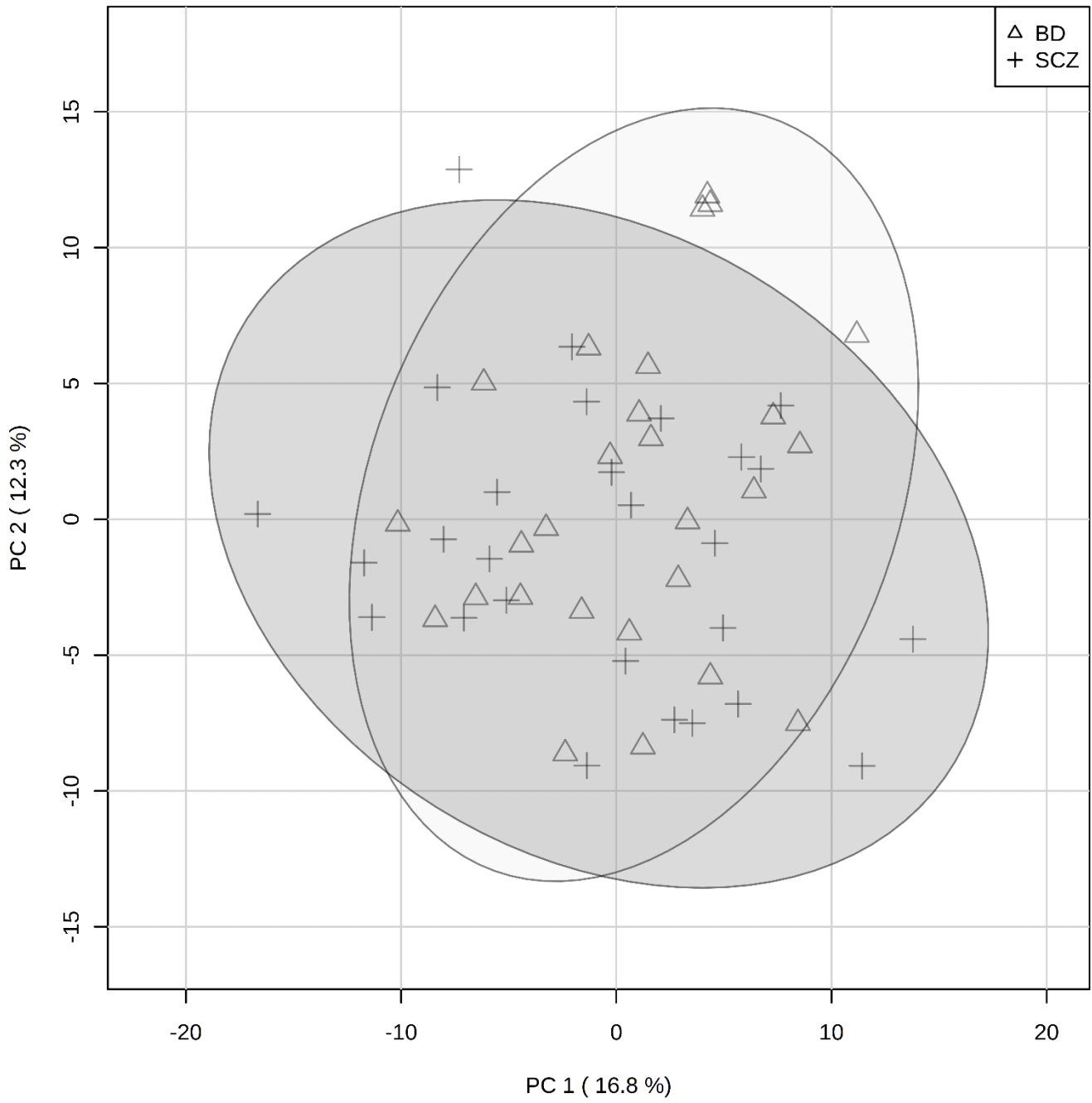
Scores Plot
