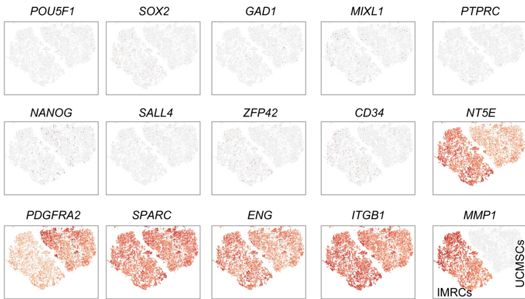
Fig. S4 IMRCs possess unique gene expression characteristics.
