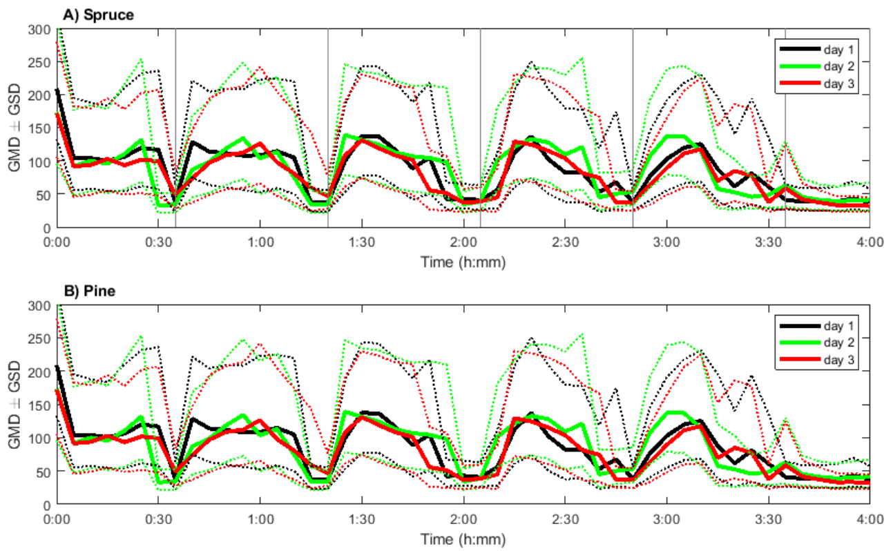
Supplementary Figure 2. Size of the particles measured by SMPS per day to day. The geometric mean diameters are shown with the solid lines, while GSDs are represented with dashed lines. (average of 3 experiments)
