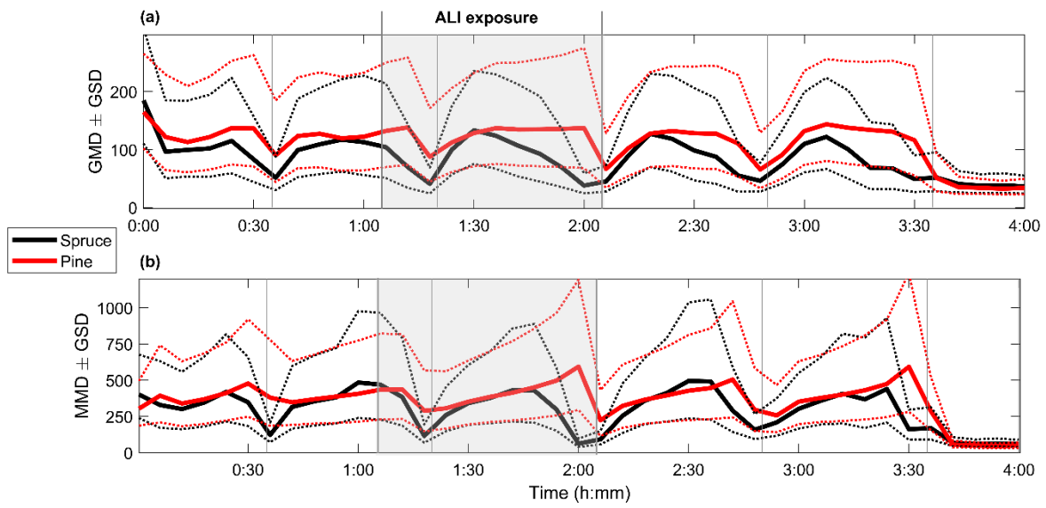
Supplementary Figure 3. Size of the particles measured by SMPS. The geometric mean diameters (a) and mass median diameters (b) are shown with the solid lines, while GSDs are represented with dashed lines. Average of 3 experiments.
