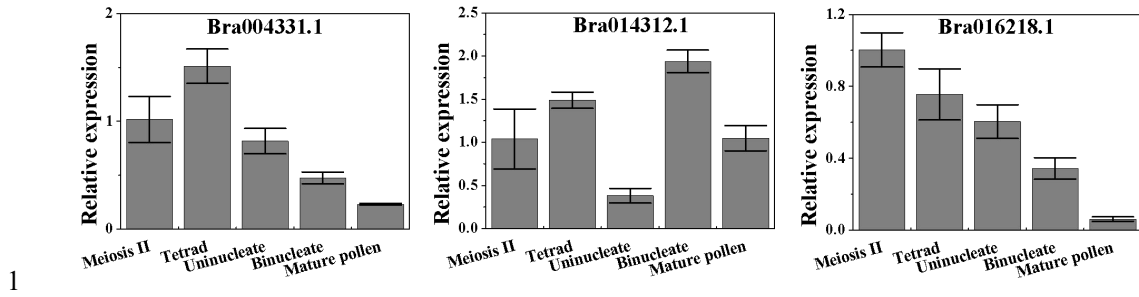
2 Fig. S8. qRT-PCR analysis of three BrPERK genes in the five periods of 3 anther development.
